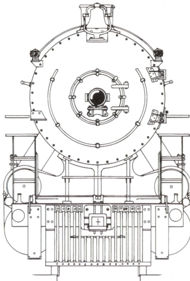
Southern Railway 2-10-2 Ss Class Drawing drawn for Mainline Modeler October 1998 by Al Armitage Used here by permission R.L. Hundman for non-commercial use ONLY
