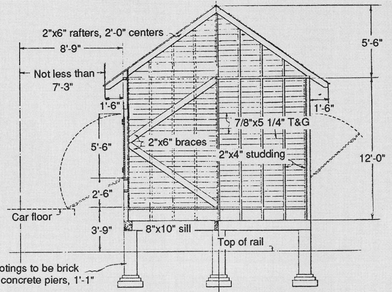
Half Cross Section - Half End Elevation
