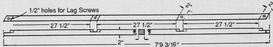
DETAIL of DIAGONAL BRACE (1-REQUIRED)
