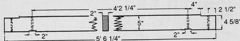
DETAIL of CROSS FRAME (4-REQUIRED)
