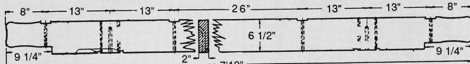
DETAIL of SIDE FRAME (2-REQUIRED)
